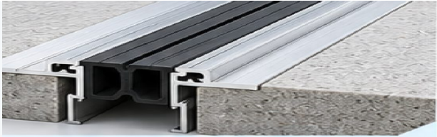
Aluminium Expansion Joint System Duty
